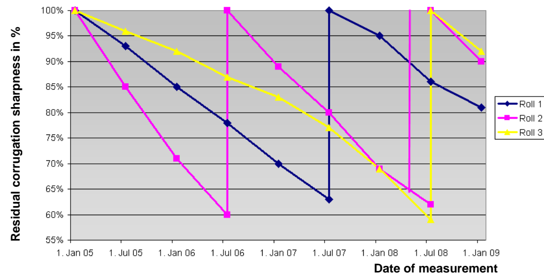
Corrugation/fluting imprint
